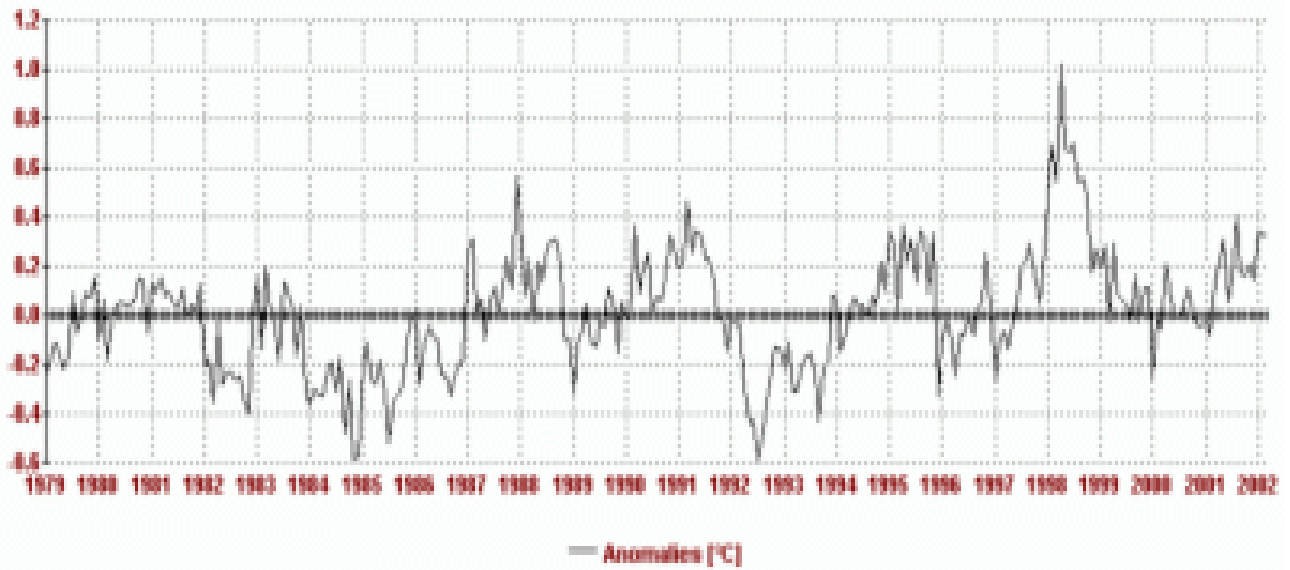
Figure 2: Northern Hemisphere Temperatures 1979-2002 legacy.abd.org.uk/climate_change_truths.htm
