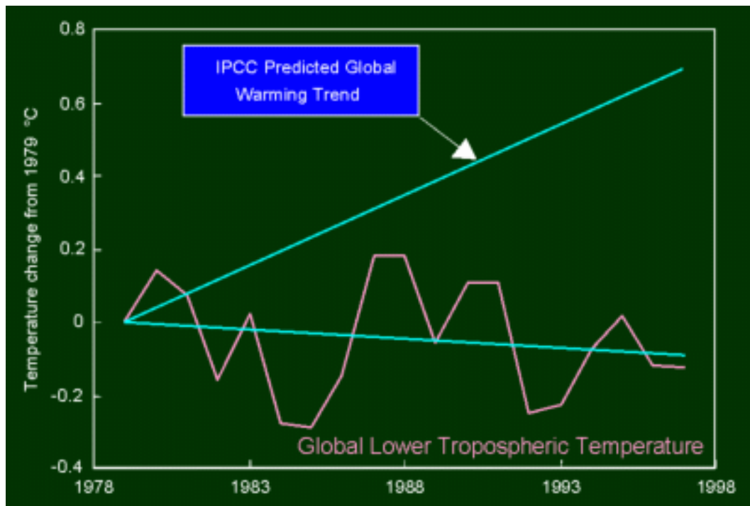
Figure 5: This graph shows troposphere temperature from satellite data against IPCC International Panel on Climate Change computer model predictions legacy.abd.org.uk/climate_change_truths.htm
