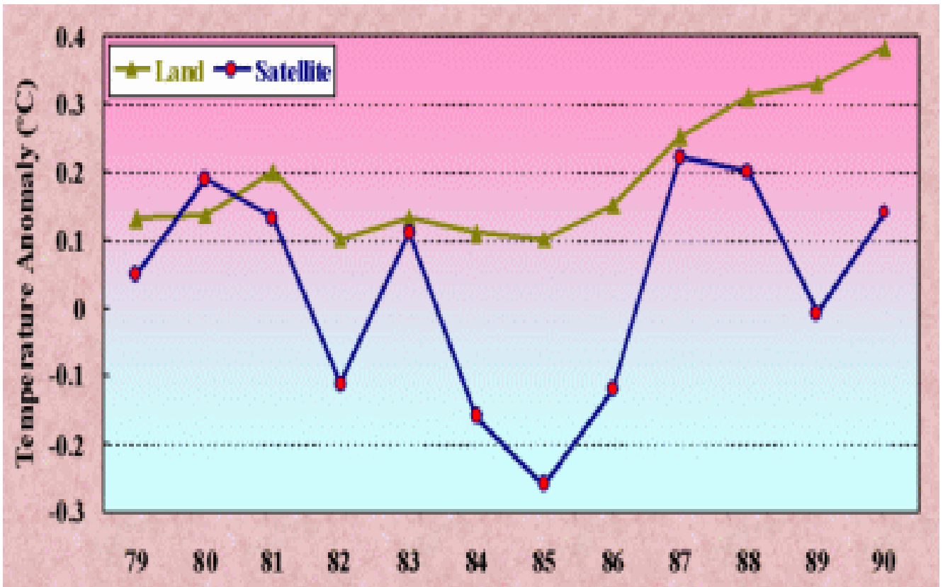
Figure 1: Comparison of Satellite and Land-based data 1979...1990 legacy.abd.org.uk/climate_change_truths.htm
